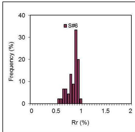
Insert the distribution of vitrinite reflectance means
